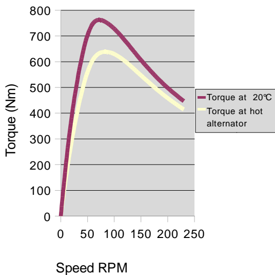
Short-circuit torque 500STK2M 150 RPM R cc = 0 Ohm
