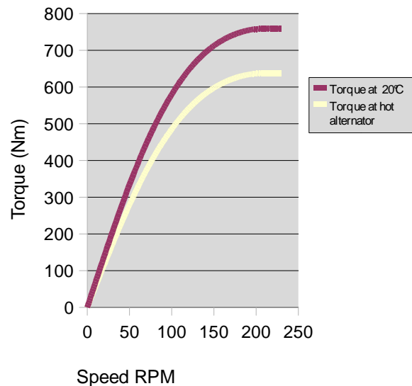
Short-circuit torque 500STK2M 150 RPM R cc = 0,25 Ohm
