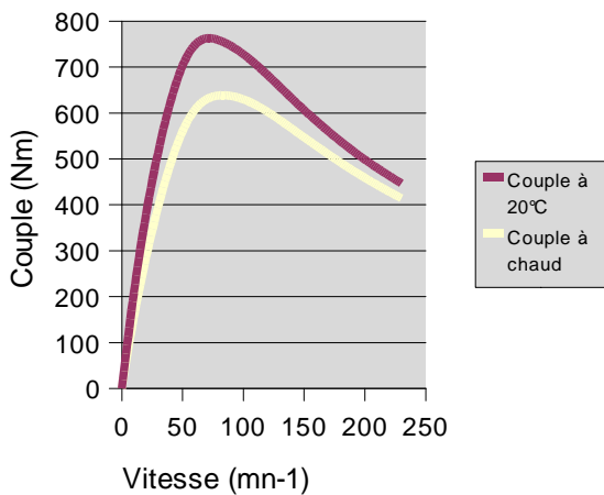
Couple court-circuit 500STK2M 150mn-1 R cc = 0 Ohm
