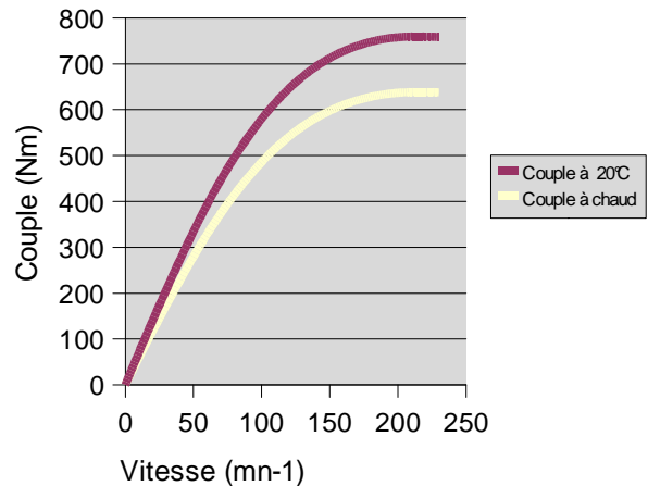
Couple court-circuit 500STK2M 150mn-1 R cc = 0,25 Ohm
