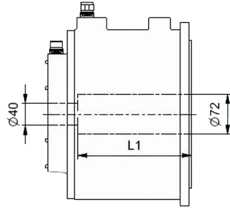
With position feedback 2, 3, 7, A or B (fig. 2)
