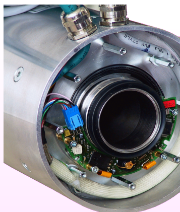
Integration of a SCS KIT 101 encoder inside a hollow shaft 145ST
